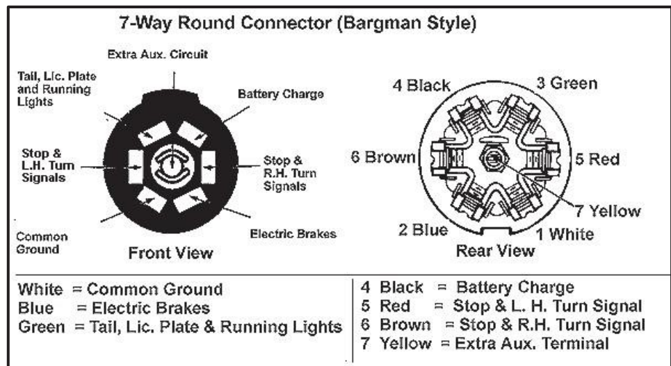
Figure 9-16: Seven-Pin Connector
