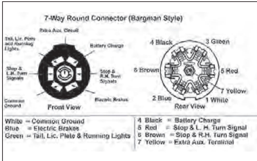
Figure 9-15: Seven-Pin towing connector
