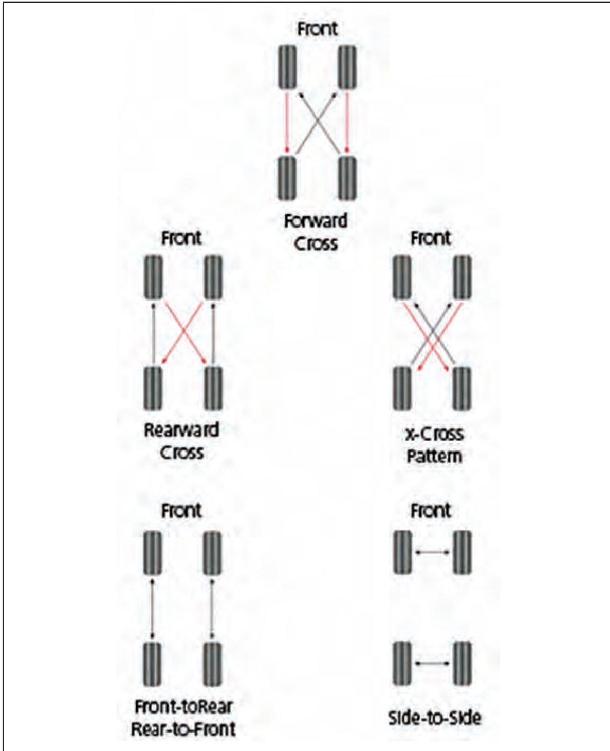
Figure 16-2: Tire rotation
