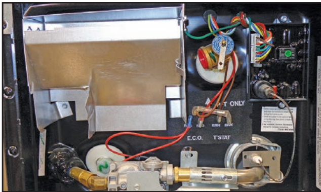
Figure 5-9: Water heater
