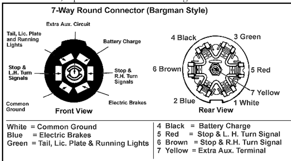
Figure 7-11. Seven-Pin Towing Connector
