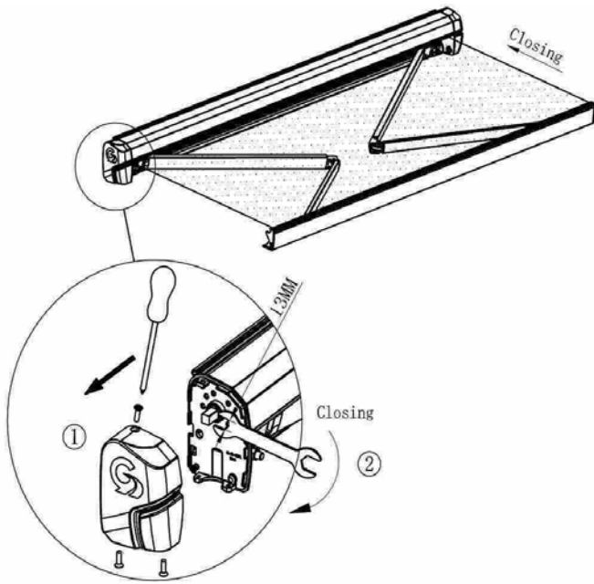
Figure 14-4: Manual Override
