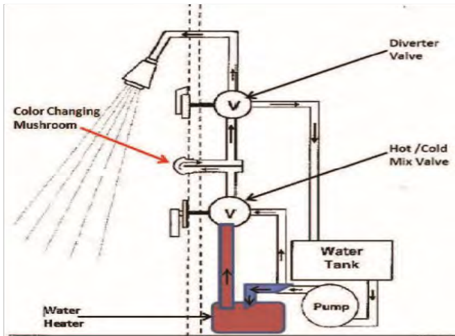
Figure 13-5: Shower Miser™ Diagram.
