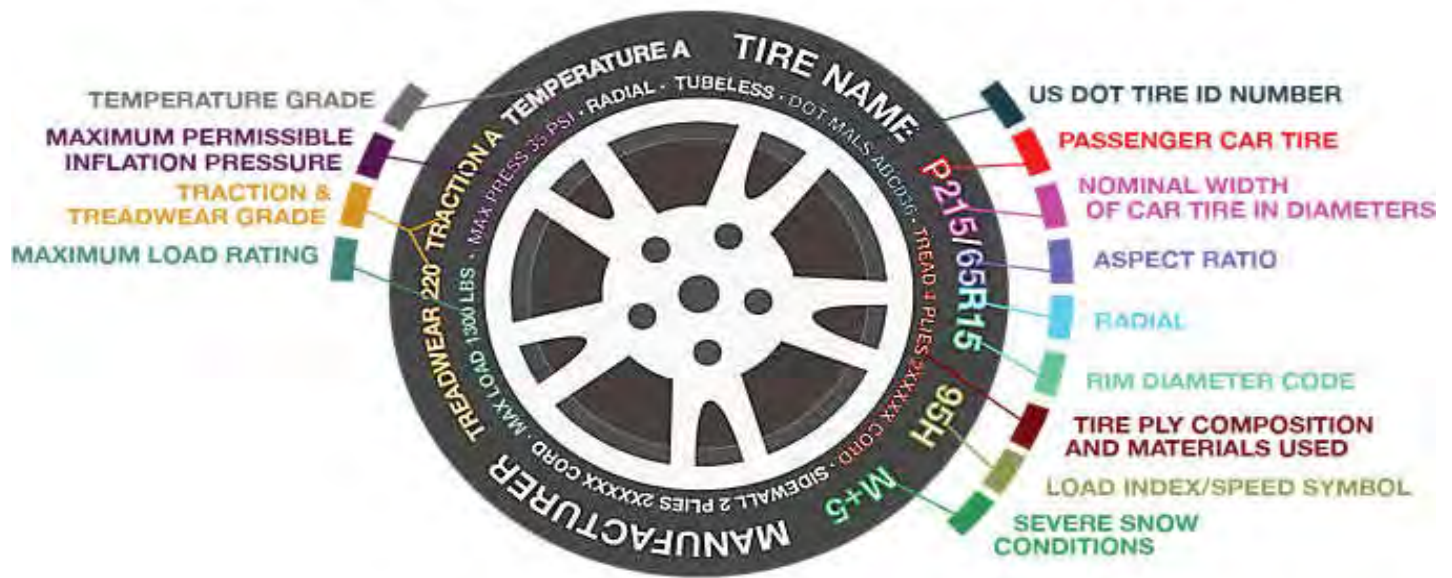
Figure 16-3: Tire Sidewall Markings
