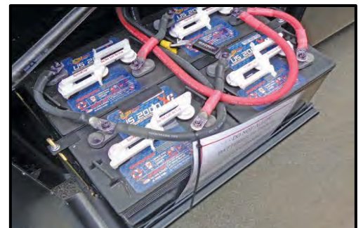
Figure 9-14: House Batteries
