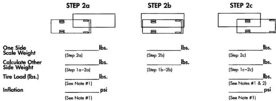
Figure 16-3: Motorhome Weighing Procedures
