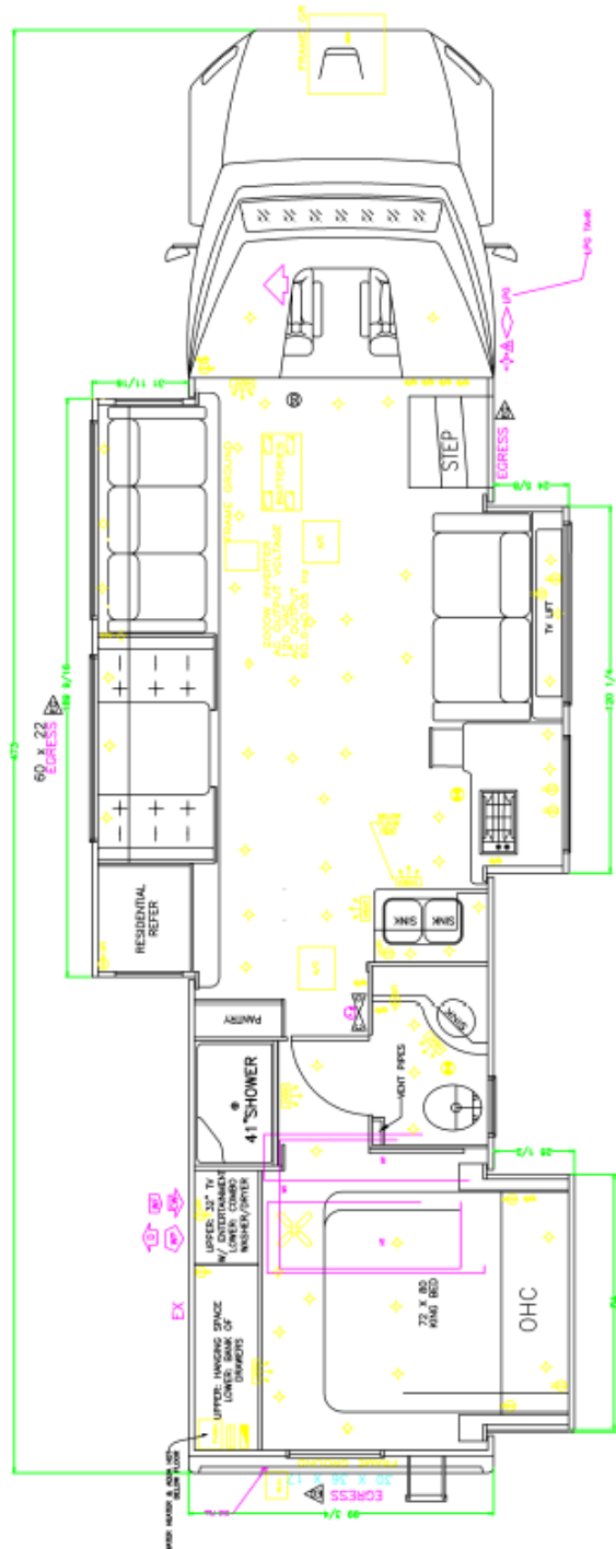
38AB Floor Plan Layout Plumbing
