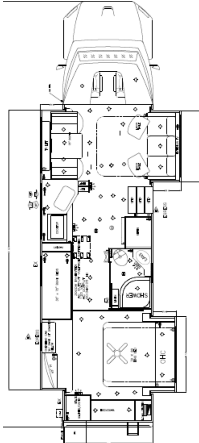
38CB Plumbing Layout
