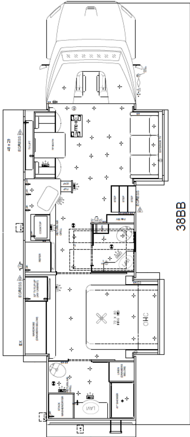
38BB Floor Plan Layout Plumbing
