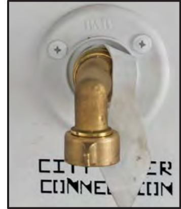
Figure 13-7: City Water Supply Connection
