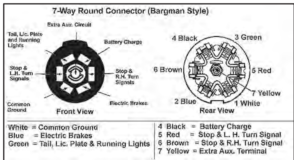
Figure 9-17: Seven-Pin Connector
