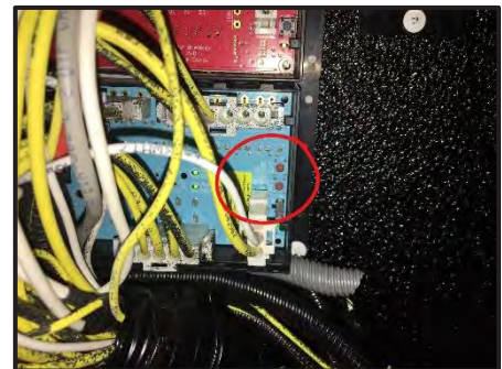
Figure 10-3: Location of Slide-Out Room Control Override
