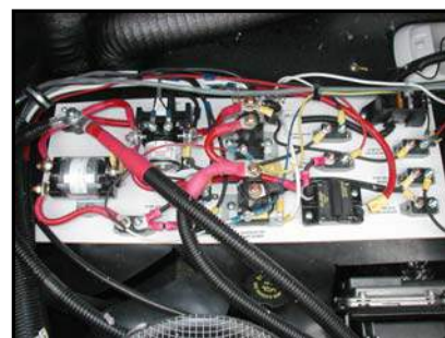
Figure 7-11. Circuit Breakers
