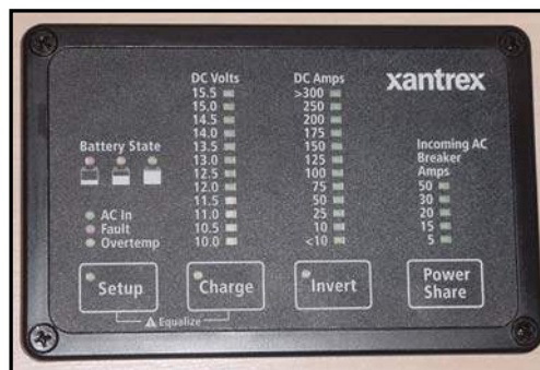
Figure 7-10. Inverter Control Panel
