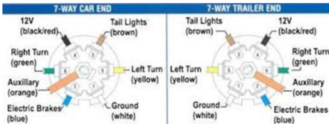
Fig. 9-18: Connection Diagram
