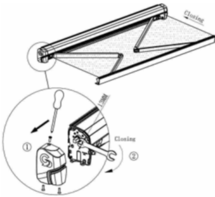
Fig. 14-2: Manual Closing the Awning
