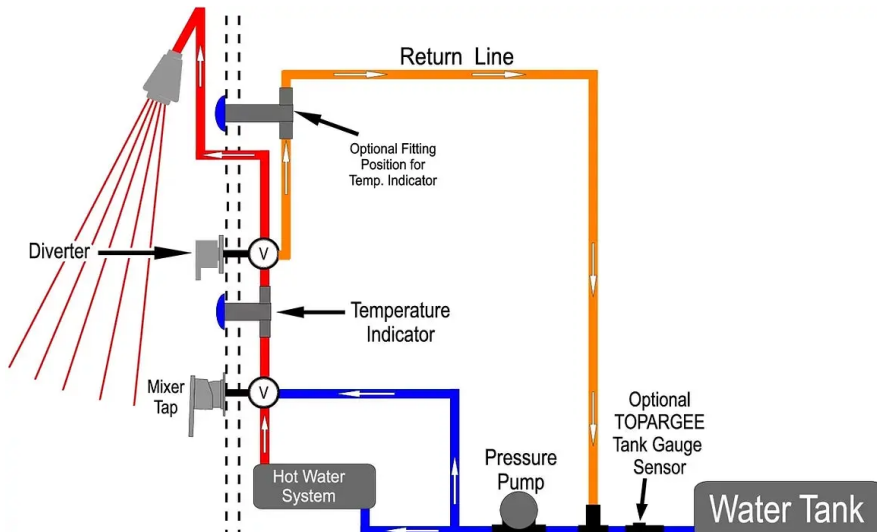
Fig. 13-6: Shower Miser™
