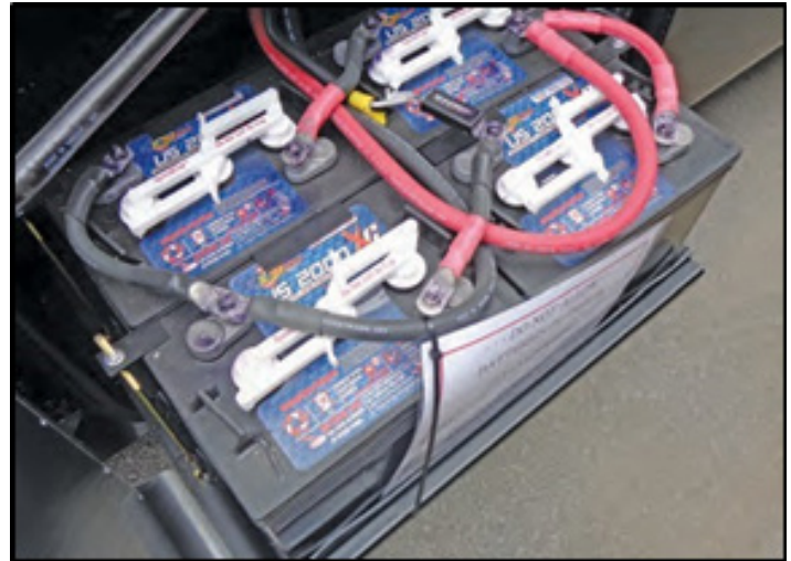
Figure 9-13: House Batteries
