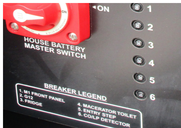
Fig. 9-10: Circuit Breakers
