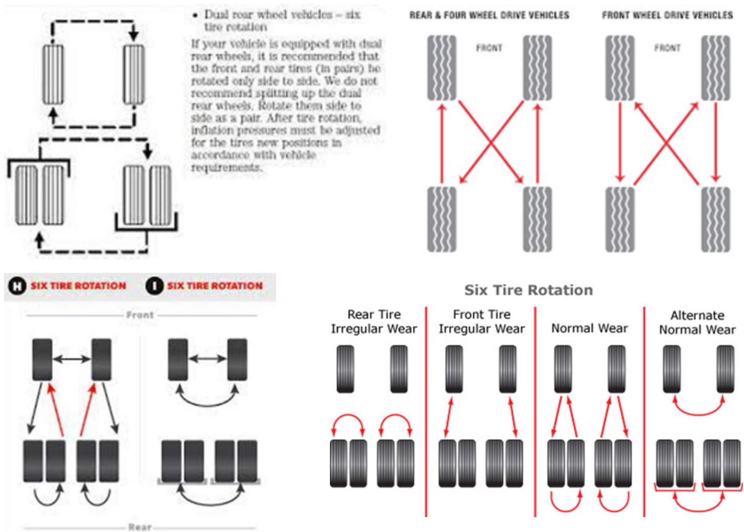
Fig. 16-1: Tire Rotation Patterns.
