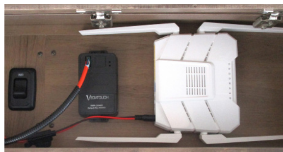
Figure 9-19: WIFI Antenna
