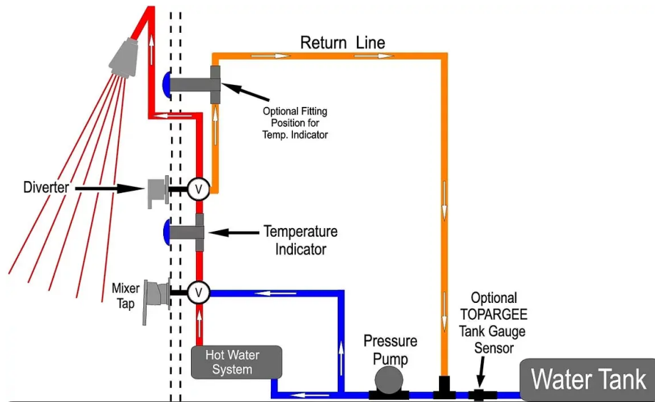
Fig. 13-6: Shower Miser
