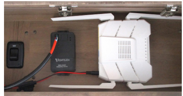
Figure 9-19: WIFI Antenna
