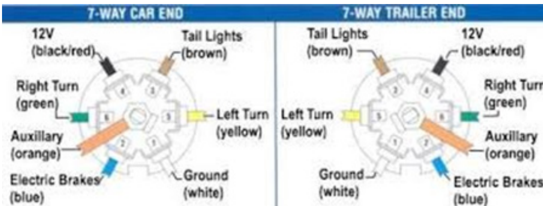
Fig. 9-18: Connection Diagram
