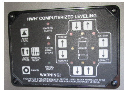
Fig. 15-5: Leveling System Controls
