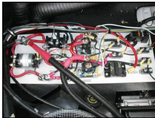
Figure 7-11. Circuit Breakers
