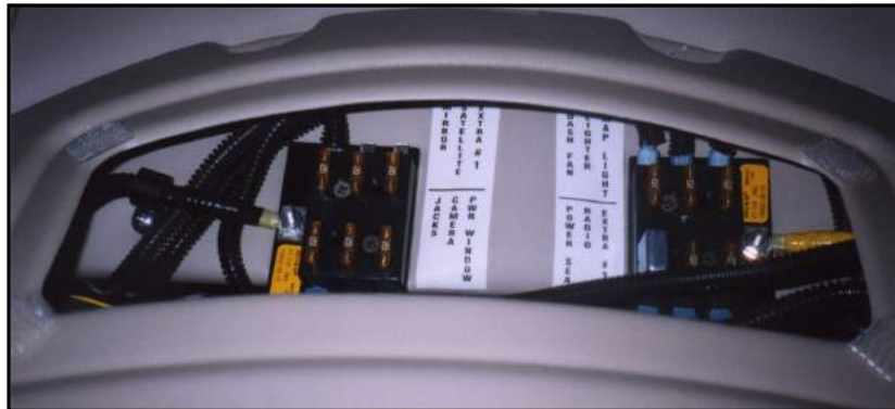
Figure 7-12. In-Dashboard Fuse Blocks
