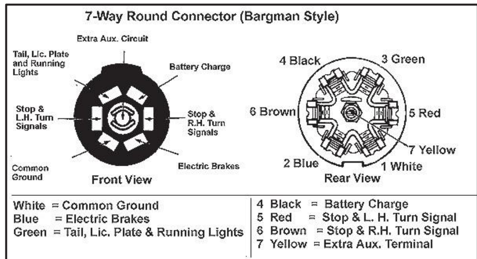
Figure 9-14: Seven-Pin Connector
