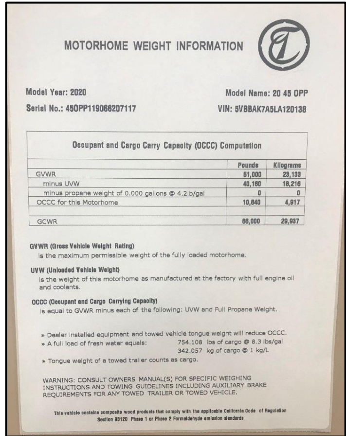
Figure 1-4: Sample Motorhome Weight Label (found in the bedroom closet)
