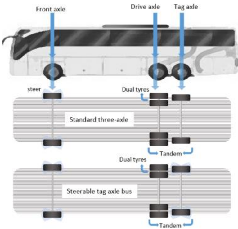
Three-axe diagram from the side and underneath perspectives
