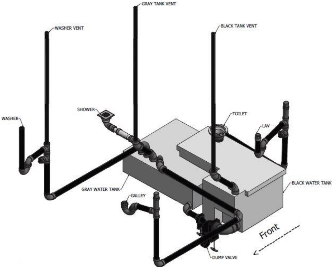
Drain Line
