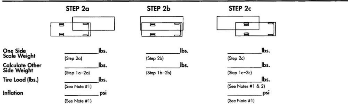
Figure 17-3: Motorhome Weighing Procedures
