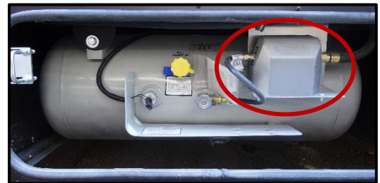
Figure 2-3: LP Gas Regulator
