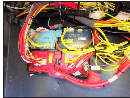
Figure 9-10: Circuit Breakers
