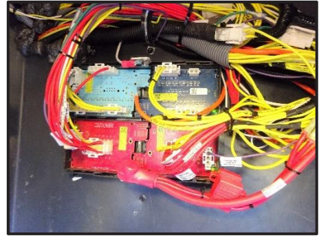
Figure 9-11: Circuit Breakers
