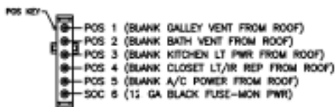
CONNECTOR 3
