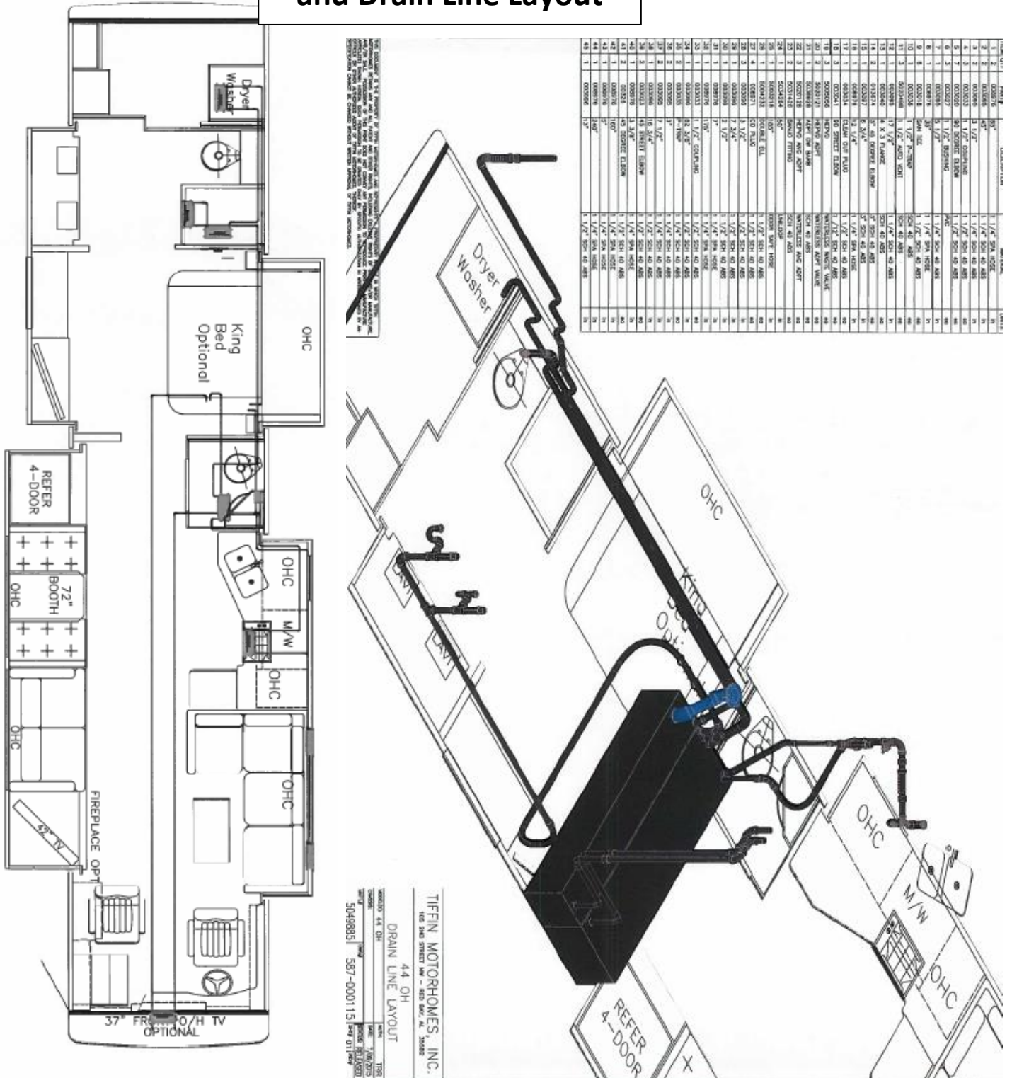
45OPP Aqua Hot Layout and Drain Line Layout
