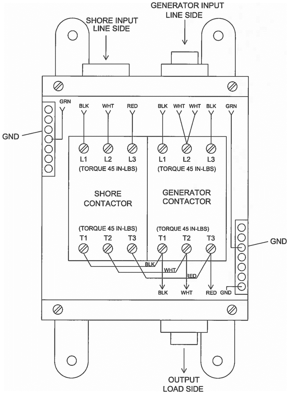
45OPP Transfer Box
