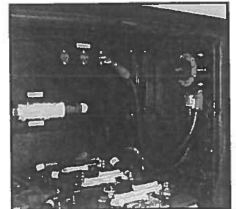
Figure 7-7. Rotary Switch to Disconnect “House” Batteries
