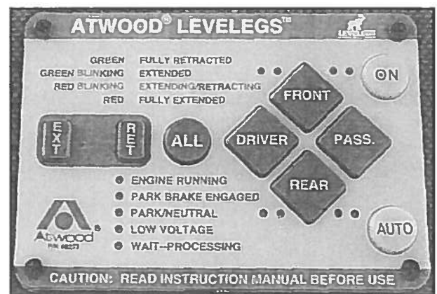
Figure 9-6. Leveling Control Panel on Dashboard
