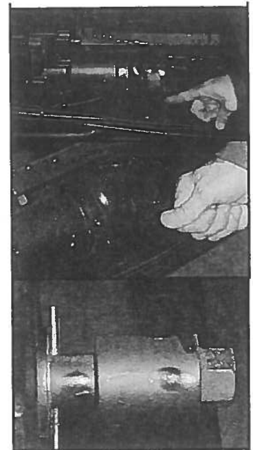
Figure 8-3. Manual Slide-Out Deployment Sequence
