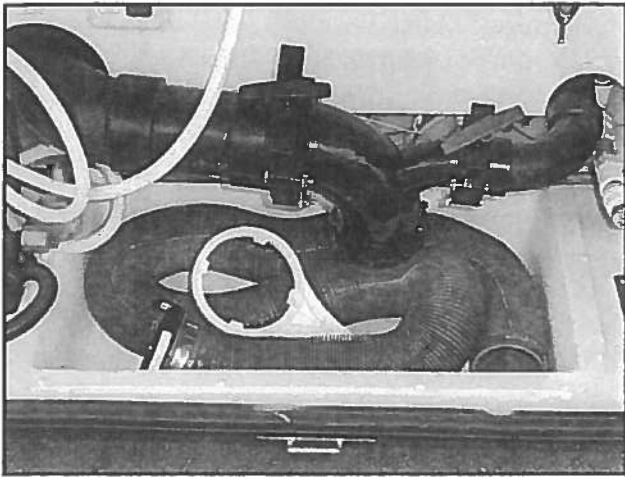
Figure 11-16. Sewer Hose and Drain Connections
