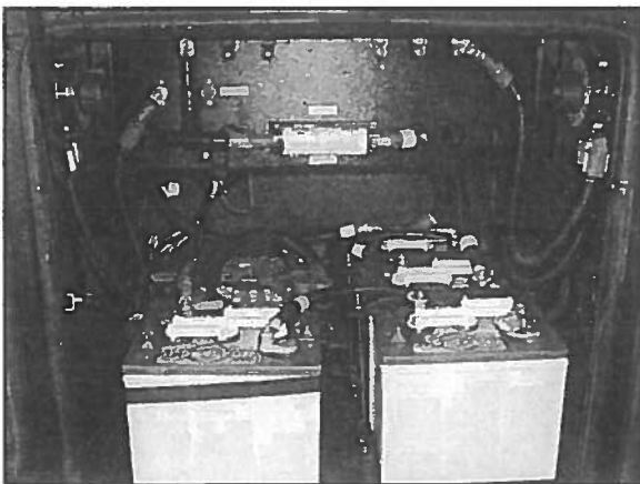
Figure 7-5. 12 VDC Battery Supply (Compartment)
