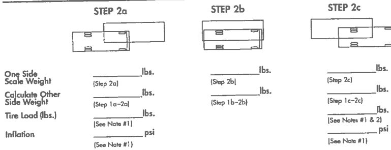
Figure 14-5. Procedure for Weighing the Motor Home (Each Tire Position Individually)
