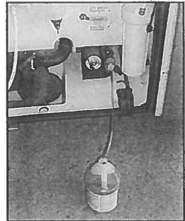
Figure 14-14. Winterizing the Water System
