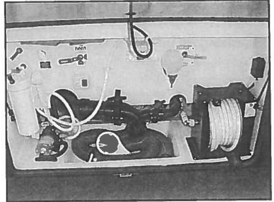
Figure 11-17. Exterior Shower in Outside Compartment
