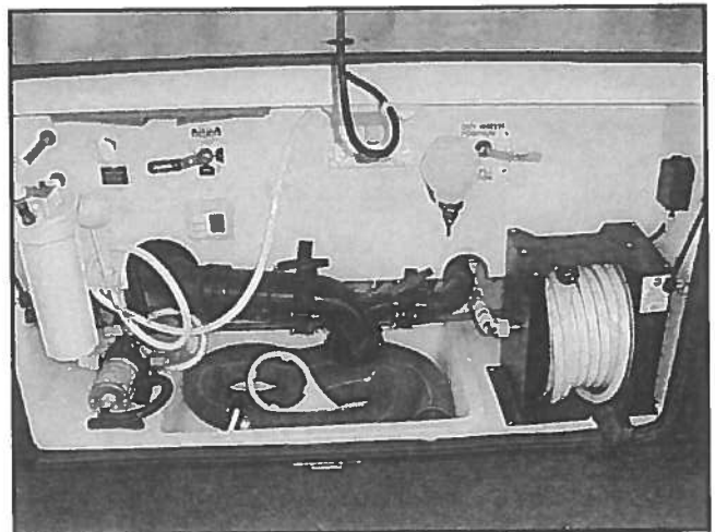
Figure 11-15. Sanitation Compartment Containing Holding Tank Drains and Flexible Drain Hose
