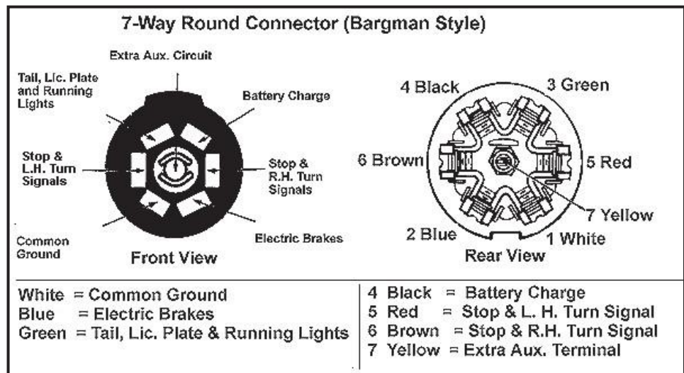
Figure 9-17: Seven-Pin Connector
