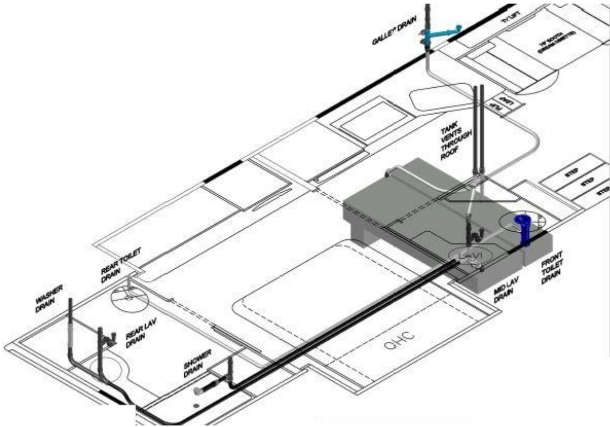
38BB Drain Line Layout
